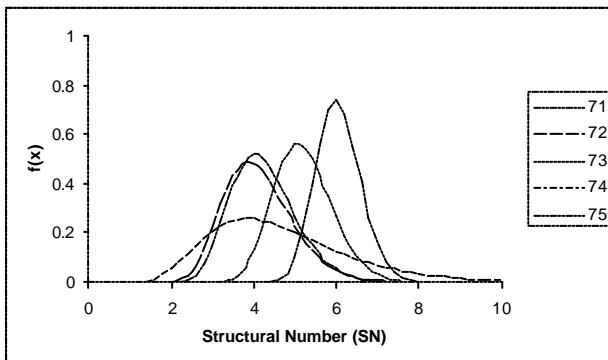
Figure A12 Probability distribution of Structural Number for kilometres of 71 to 75
