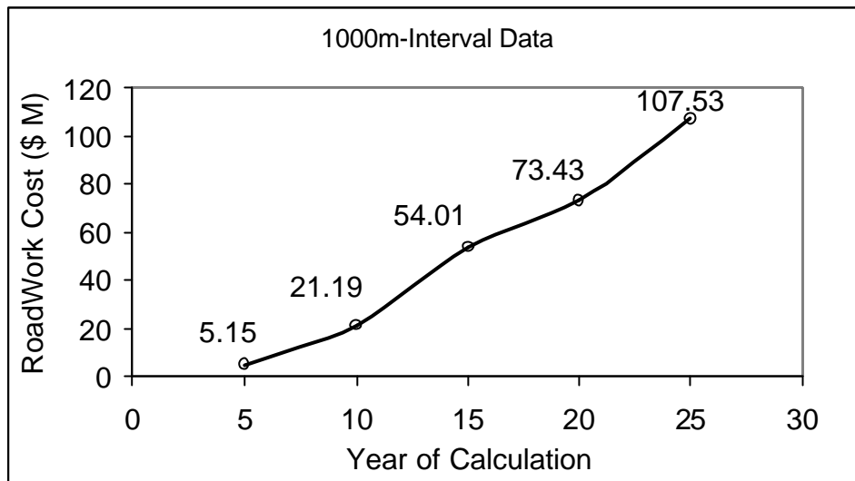
Figure 15 Budget estimates calculated from the optimal pavement deflection data of 1000-metre intervals for 5-, 10-, 15-, 20- and 25-year periods.
