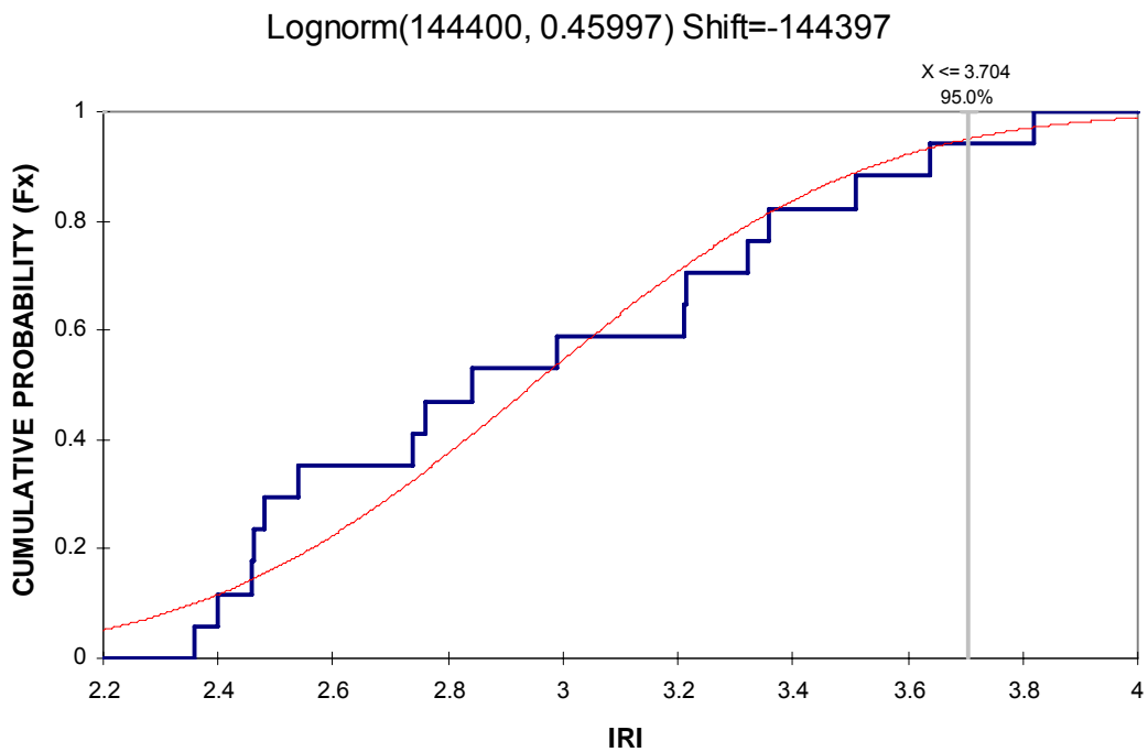
Figure A17-R17. Cumulative probability distributions of roughness for dry non reactive soil, asphalt concrete surfacing, flexible pavement, 2.31 < IRI < 4.2, AADT=501-1500 (DNR-Fair-AC-Flx-(0.5k-1.5k))
