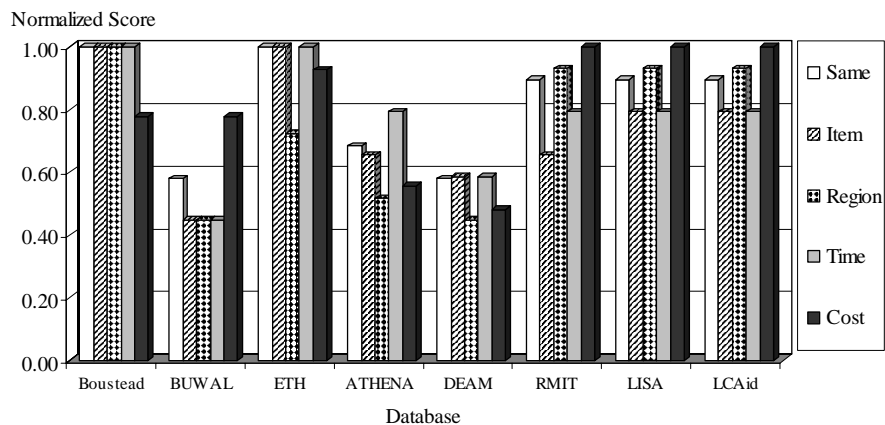
Figure 4 Comparison of selected databases with normalisation value (Best value = 1)
