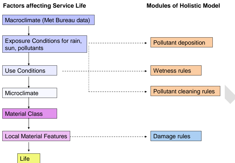
Figure 2. Factors affecting service life of metallic components and how they relate to modules of the holistic model.
