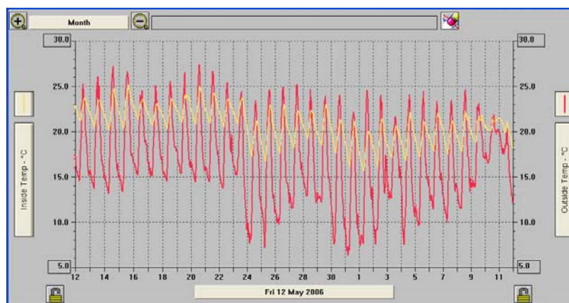
Figure 6-3 Case study 5 – external (lot) and internal (dwelling) temperatures May 2006
