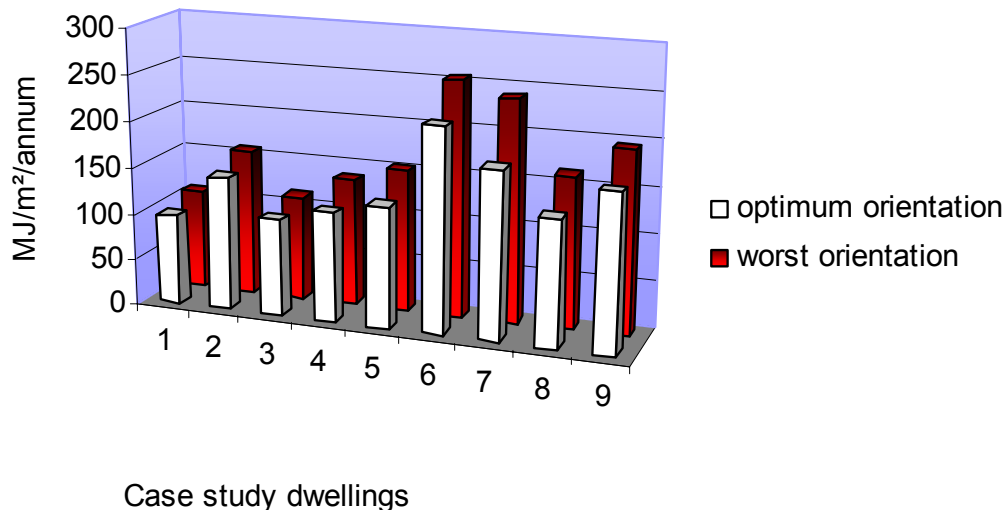
Figure 2-11 Impact of orientation on dwelling energy efficiency
