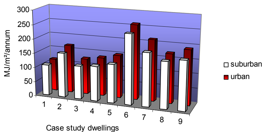
Figure 2-14 Impact of increased external shielding on energy efficiencies
