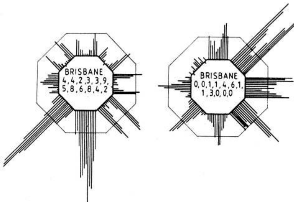
Figure 2-12 Brisbane wind rose for 9AM and 3PM
