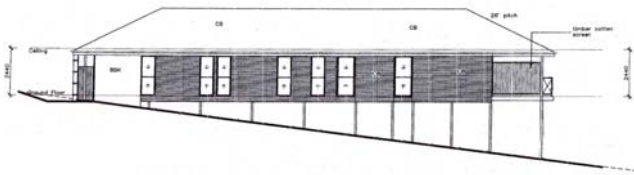
Case study 2 – single storey, elevated, metal clad, metal roof, 150m 2 internal space with 3 bedrooms, 2 pedestals
