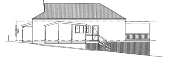
Case study 7 - split level, clad, metal roof, 263m 2 internal space with 3 bedrooms, 2 pedestals
